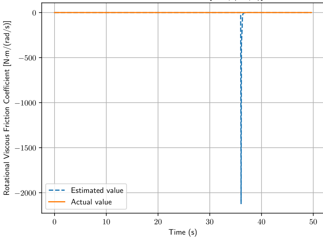
Rotational Viscous Friction Coefficient [ \text{N}\cdot\text{m}/(\text{rad}/\text{s}) ] Over Time
